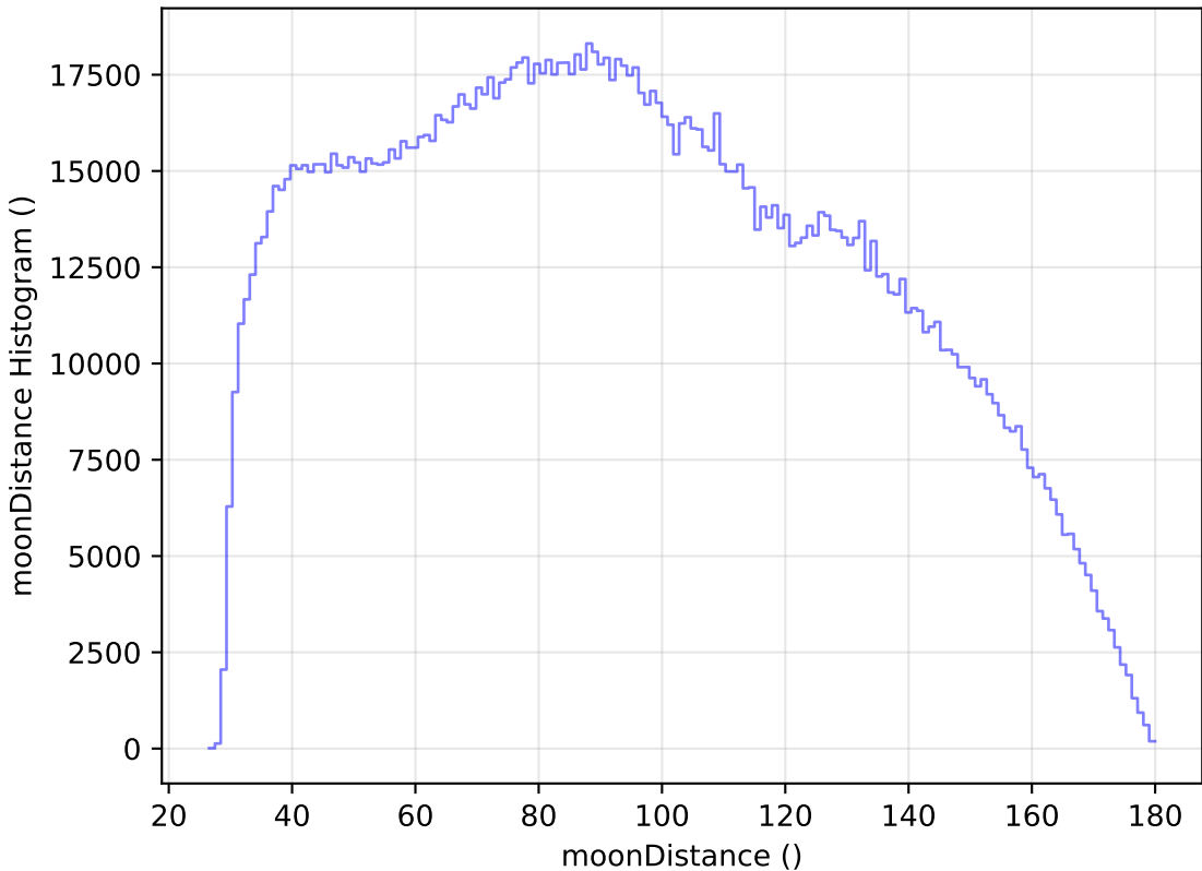
baseline_v2.0_10yrs All sky all bands: moonDistance Histogram
