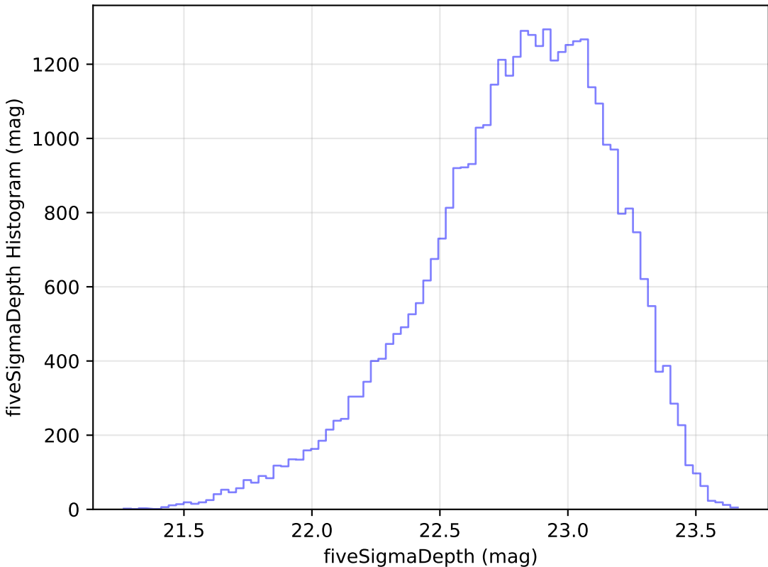
baseline_v2.0_10yrs Yr 1 z band: fiveSigmaDepth Histogram
