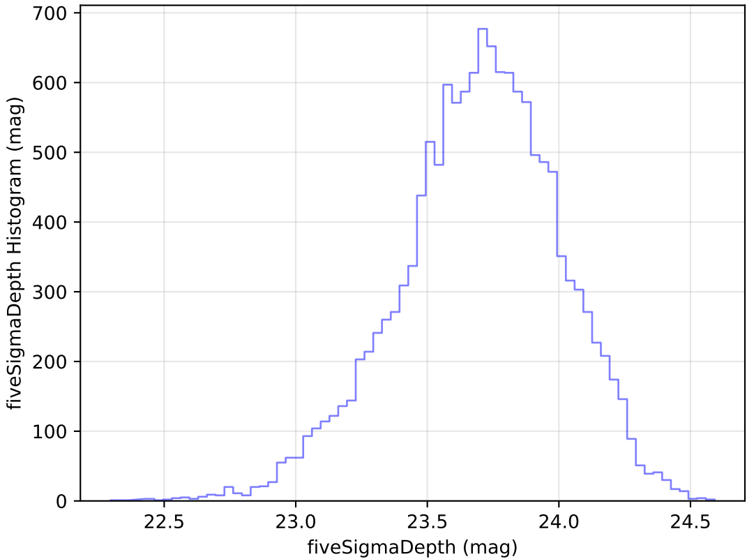
baseline_v2.0_10yrs Yr 1 u band: fiveSigmaDepth Histogram
