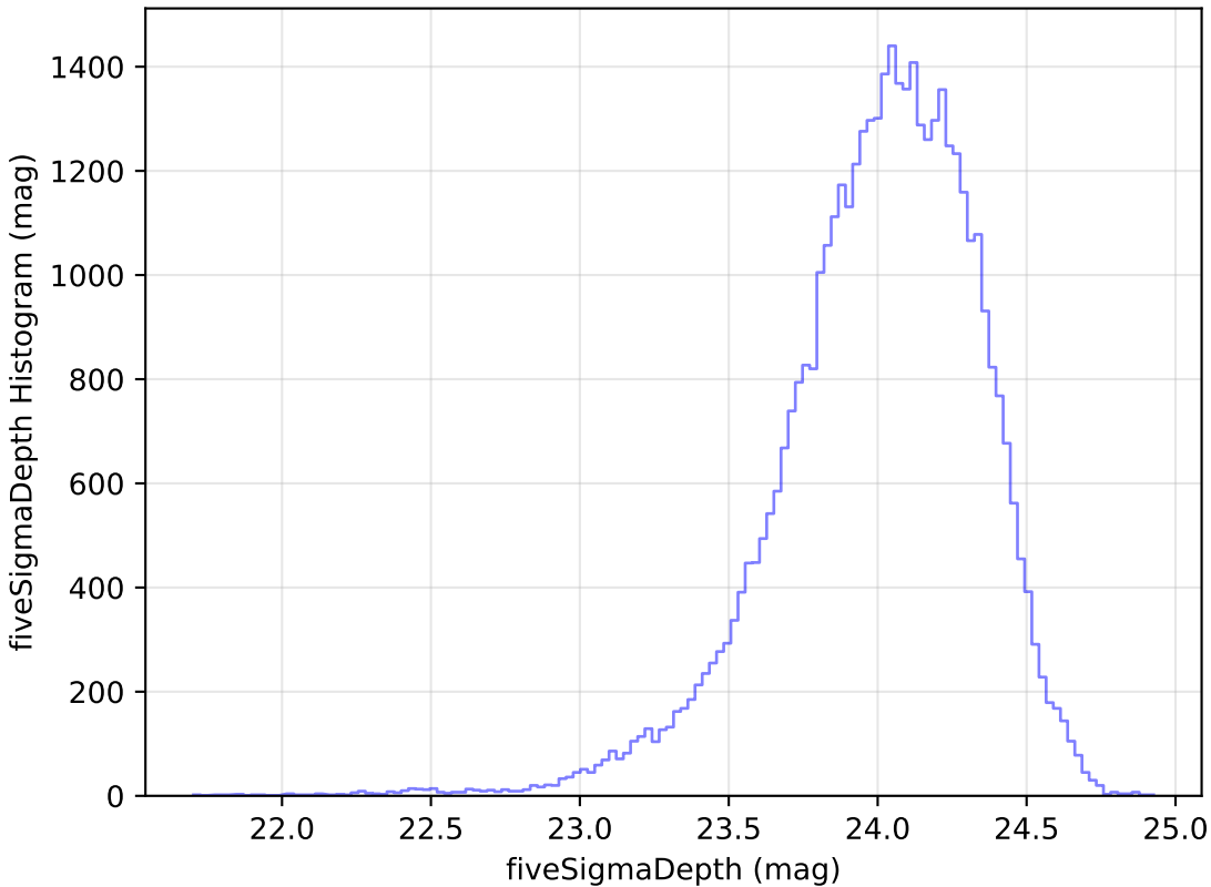
baseline_v2.0_10yrs Yr 1 r band: fiveSigmaDepth Histogram
