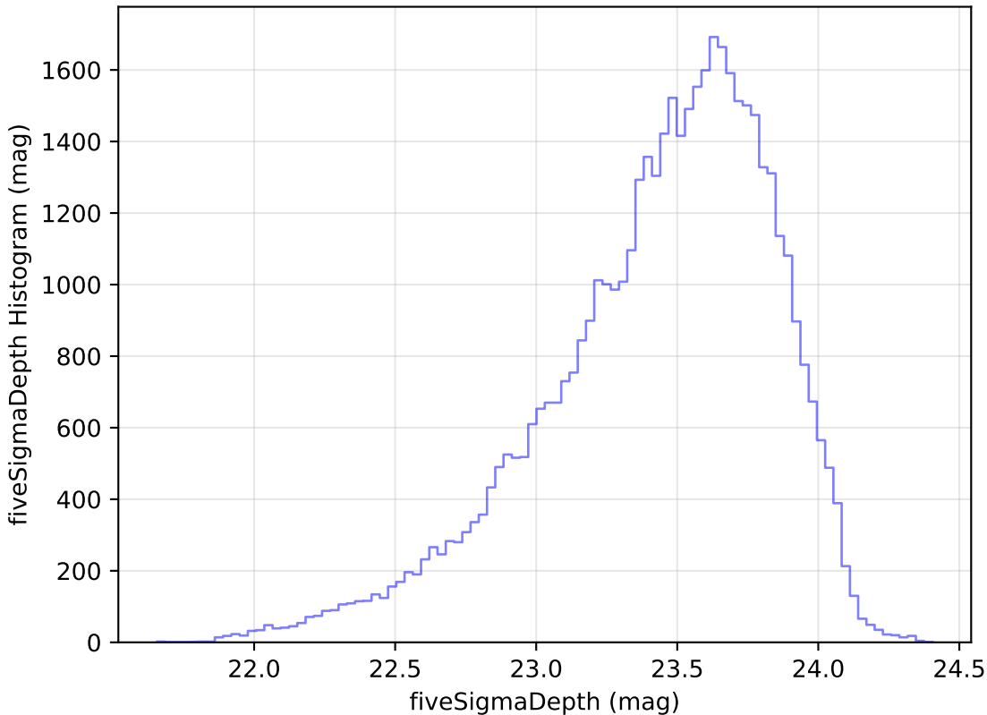
baseline_v2.0_10yrs Yr 1 i band: fiveSigmaDepth Histogram
