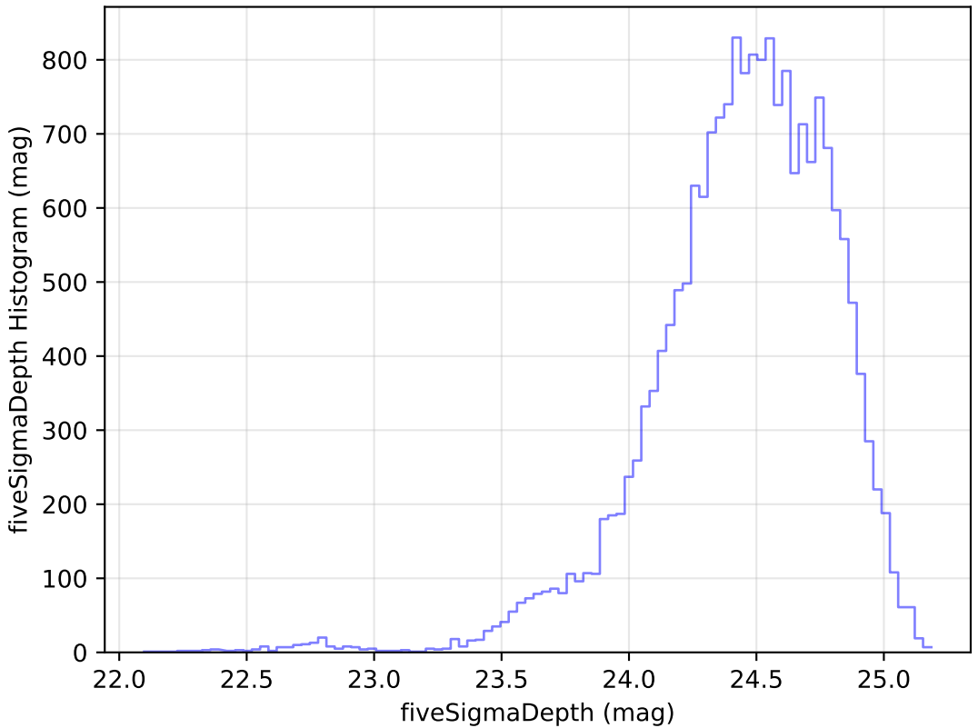
baseline_v2.0_10yrs Yr 1 g band: fiveSigmaDepth Histogram
