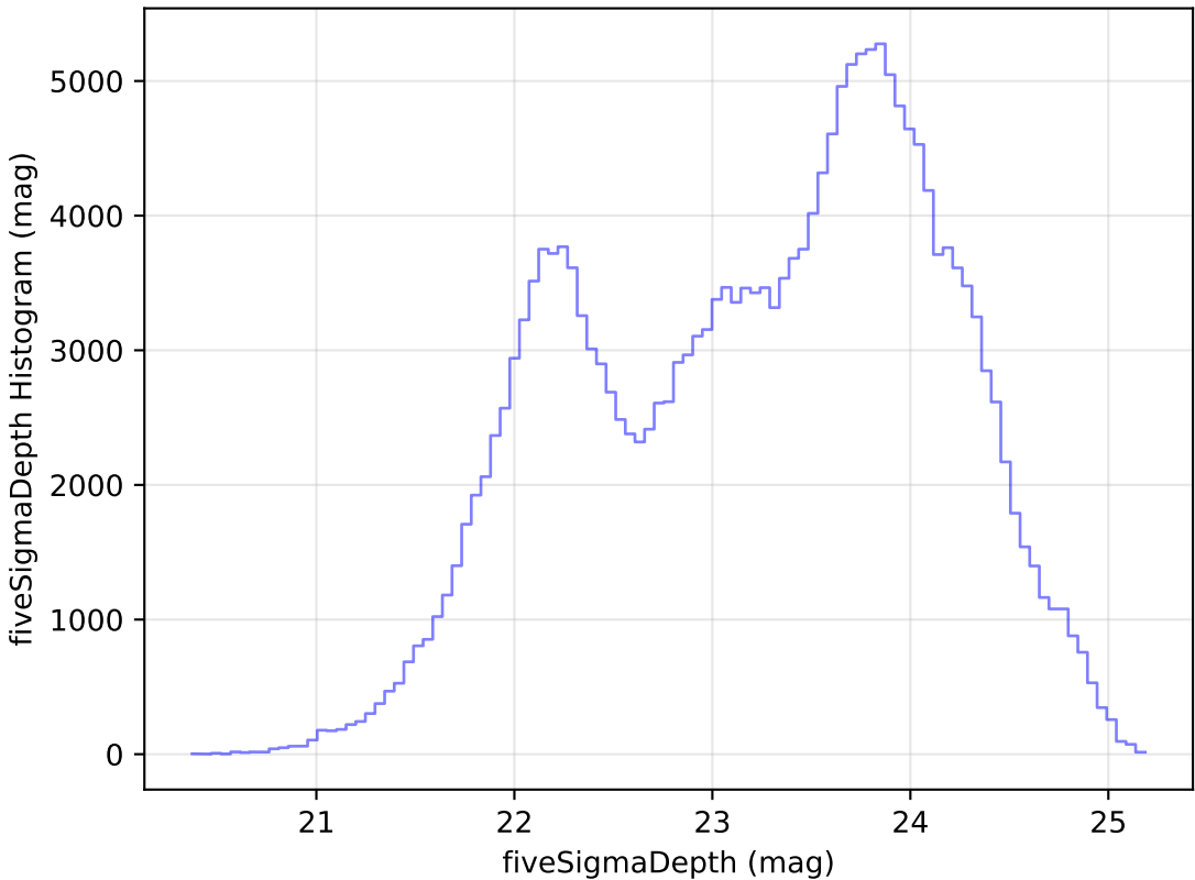
baseline_v2.0_10yrs Yr 1 all bands: fiveSigmaDepth Histogram
