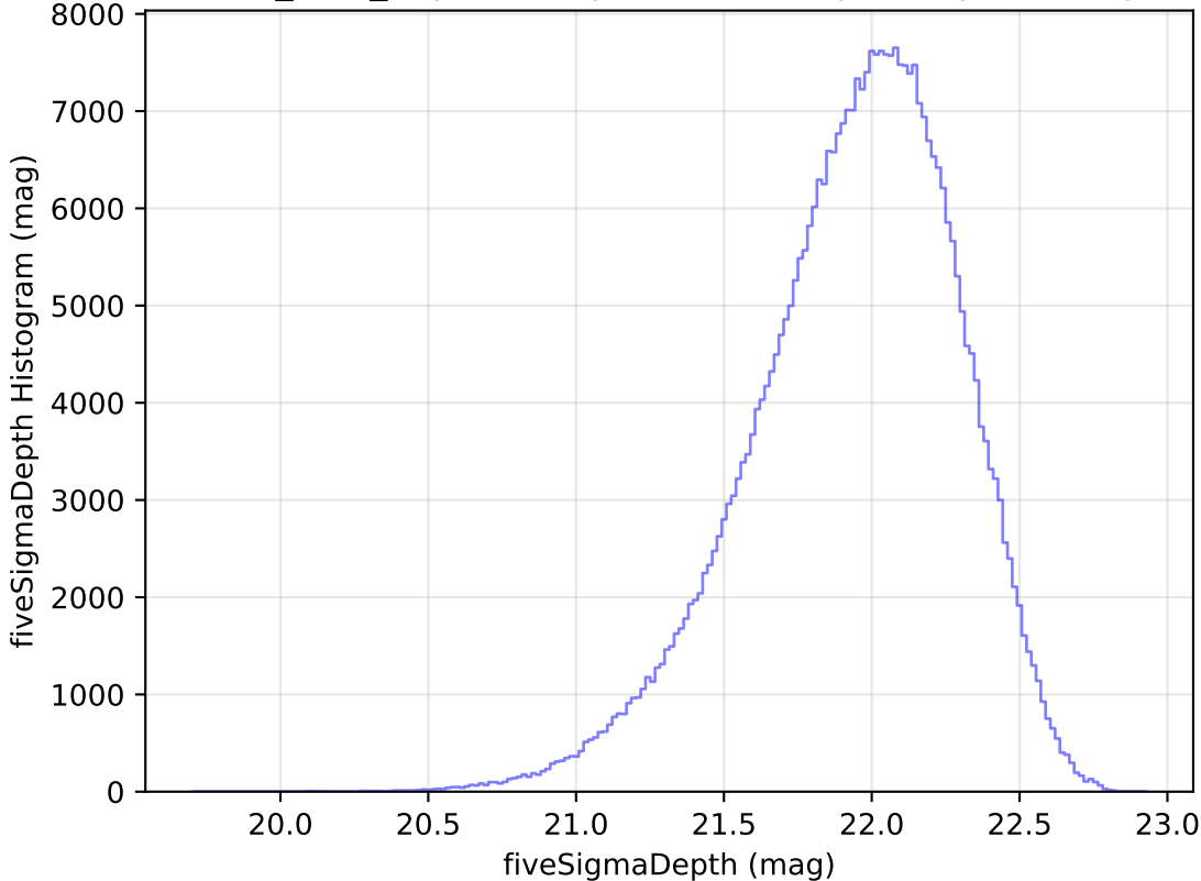
baseline_v2.0_10yrs WFD y band: fiveSigmaDepth Histogram
