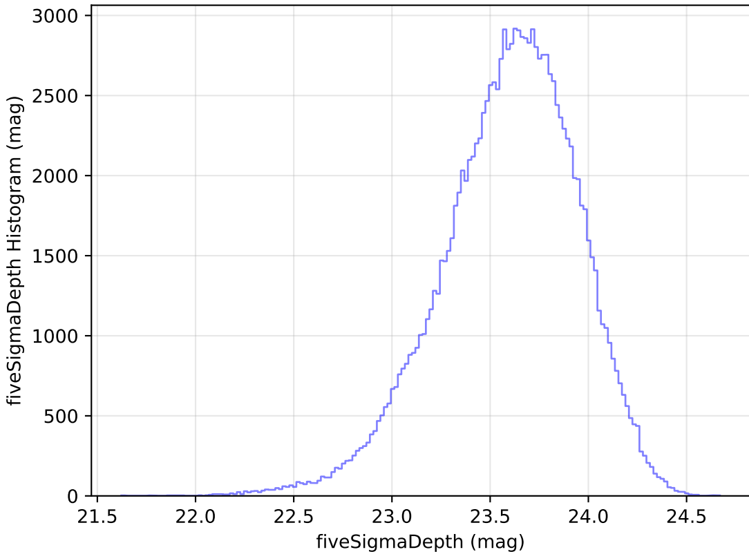
baseline_v2.0_10yrs WFD u band: fiveSigmaDepth Histogram
