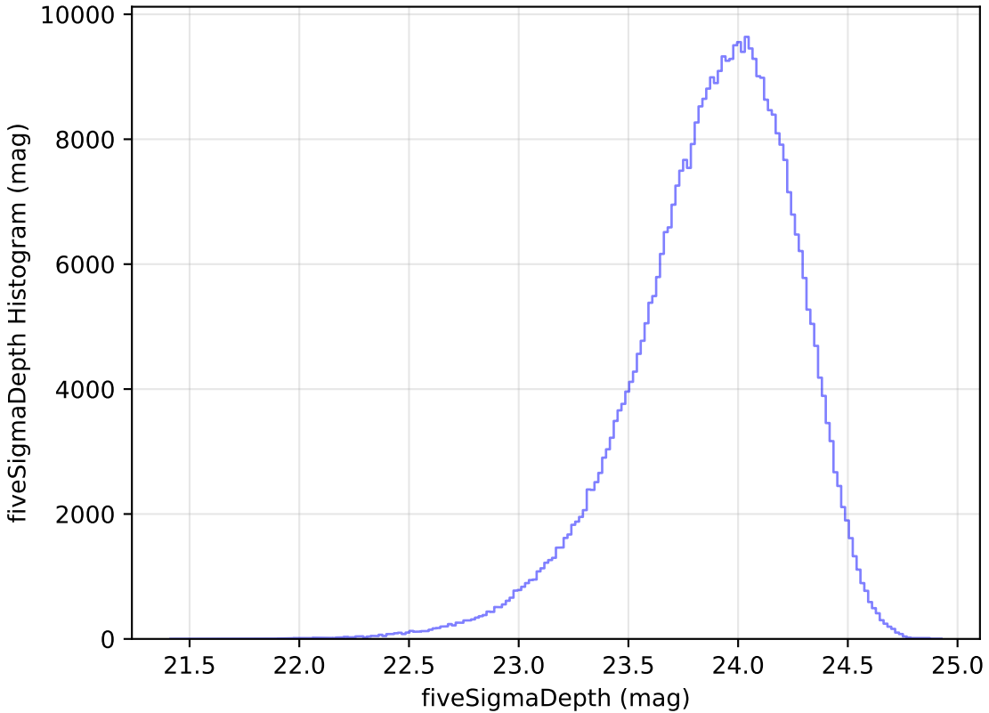
baseline_v2.0_10yrs WFD r band: fiveSigmaDepth Histogram
