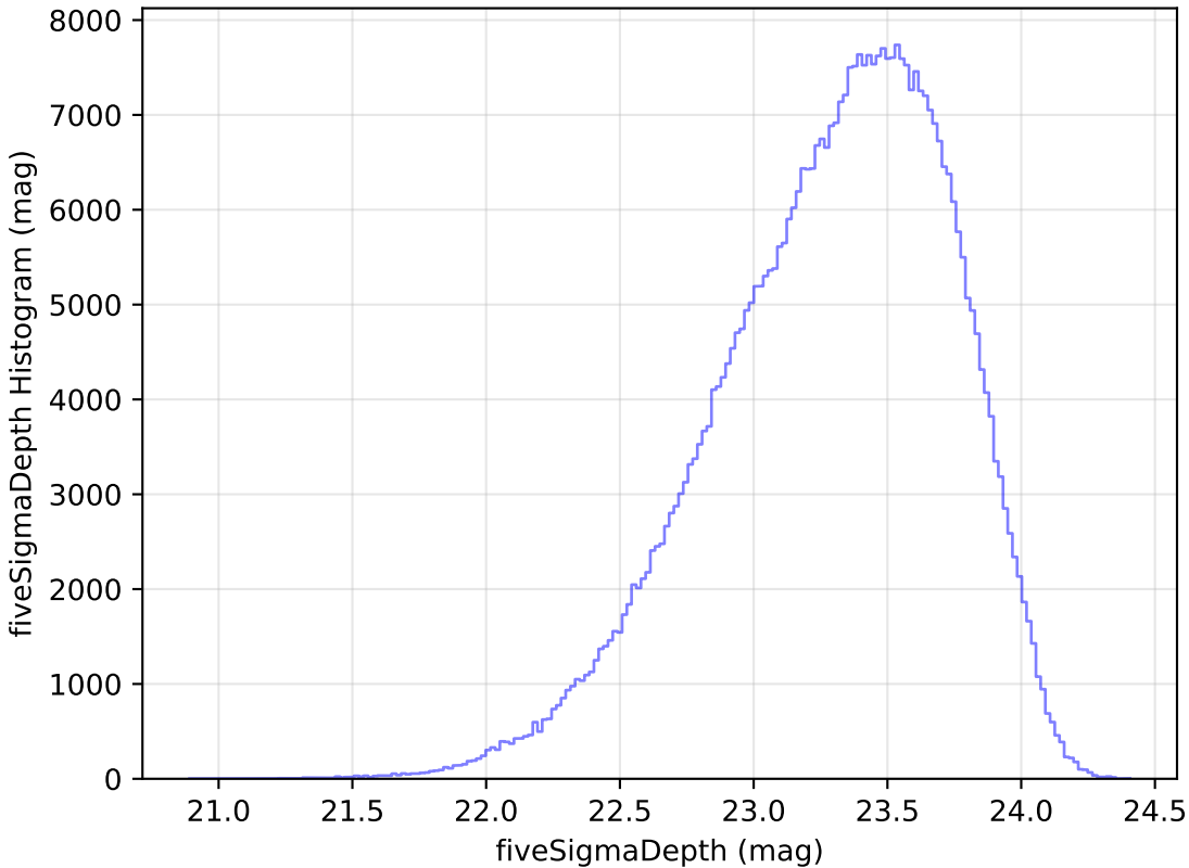
baseline_v2.0_10yrs WFD i band: fiveSigmaDepth Histogram
