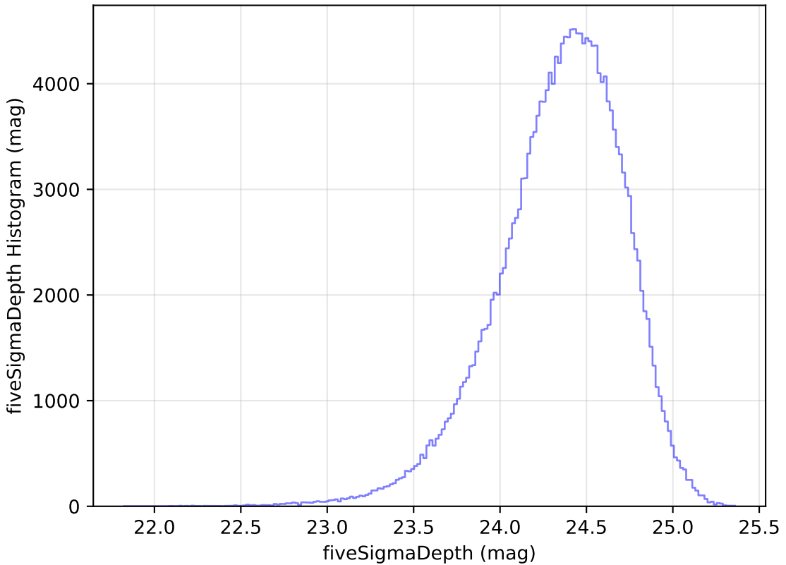
baseline_v2.0_10yrs WFD g band: fiveSigmaDepth Histogram
