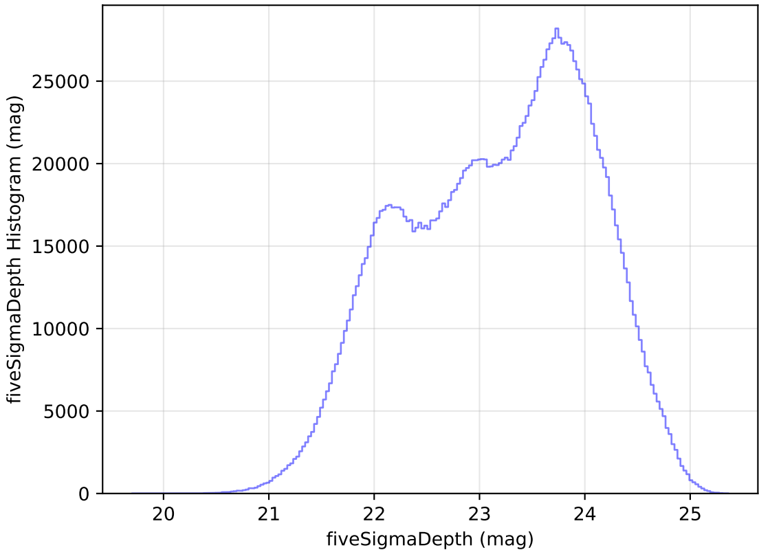
baseline_v2.0_10yrs WFD all bands: fiveSigmaDepth Histogram
