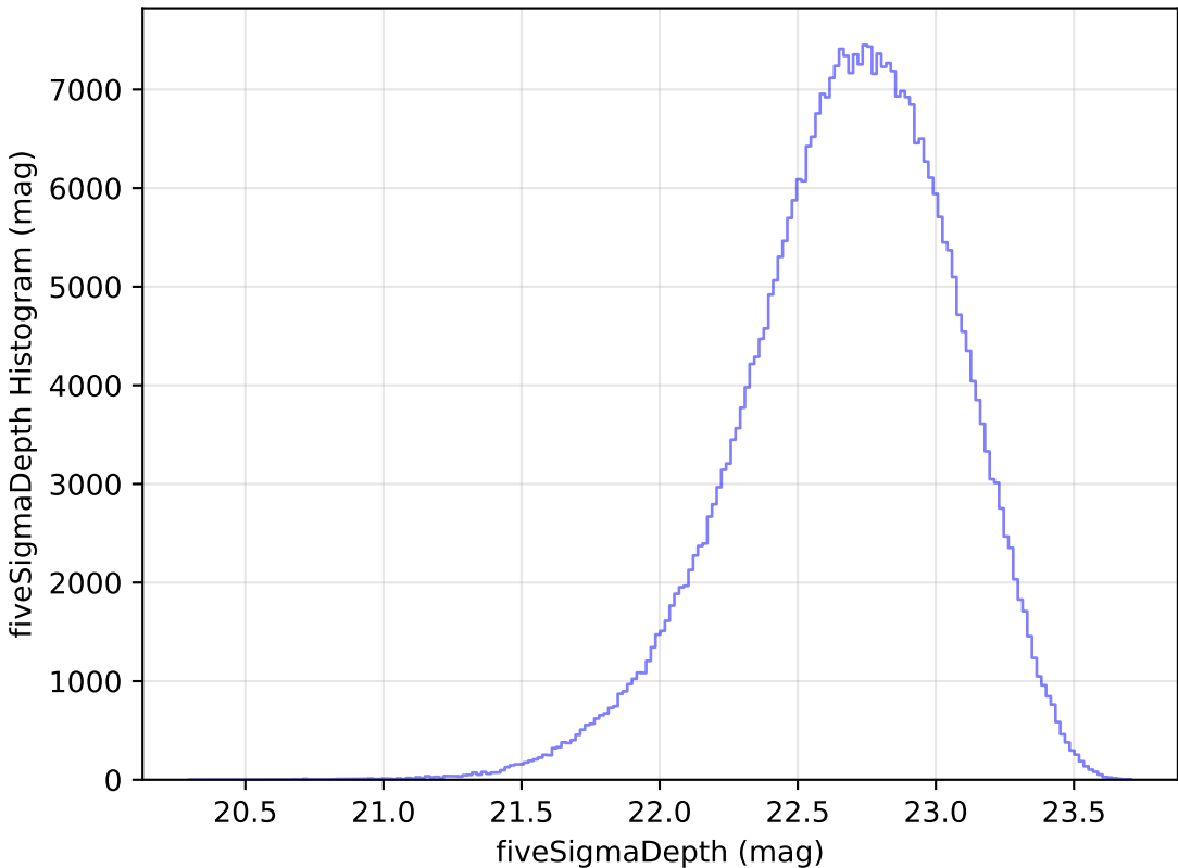
baseline_v2.0_10yrs All sky z band: fiveSigmaDepth Histogram
