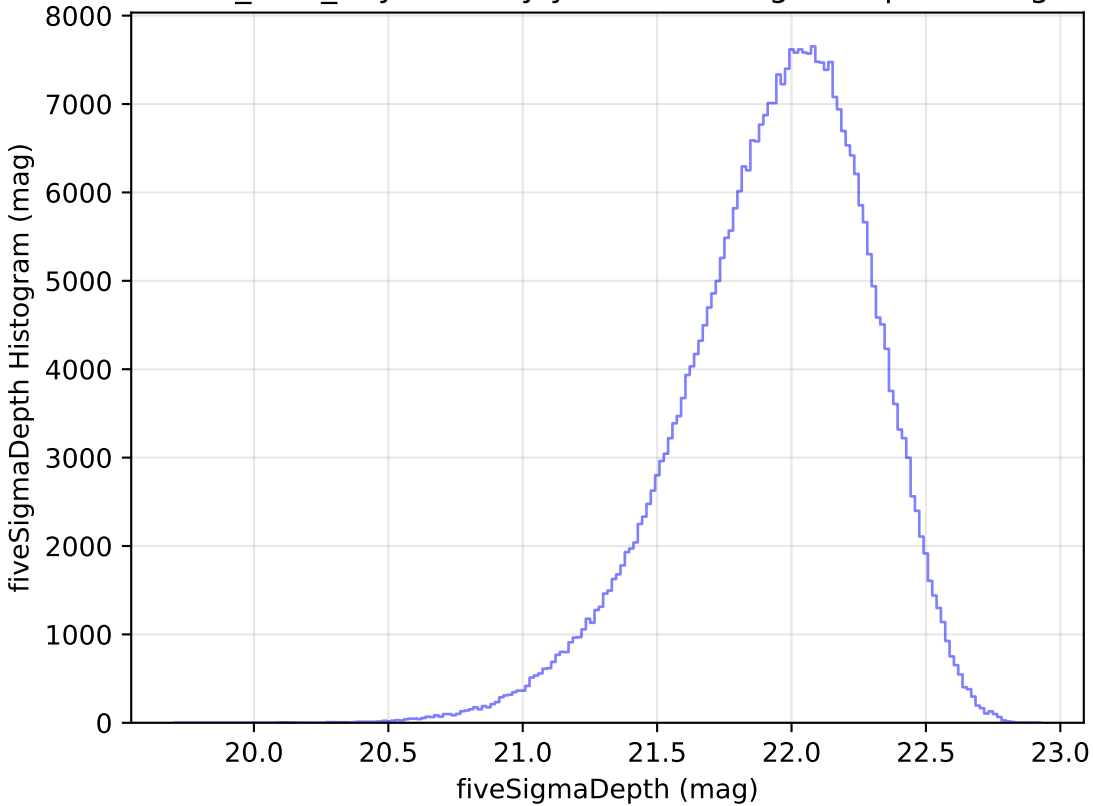
baseline_v2.0_10yrs All sky y band: fiveSigmaDepth Histogram
