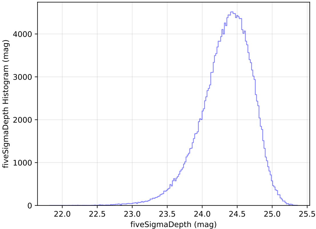
baseline_v2.0_10yrs All sky g band: fiveSigmaDepth Histogram
