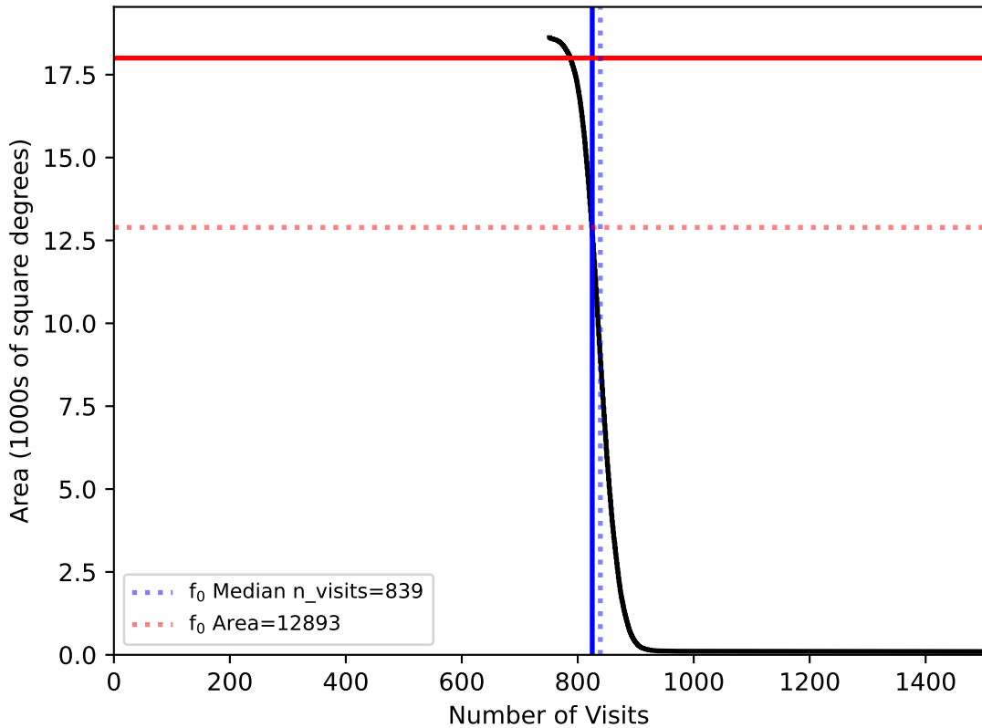
baseline_v2.0_10yrs WFD: f0
