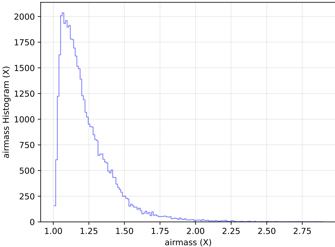
baseline_v2.0_10yrs Yr 1 y band: airmass Histogram
