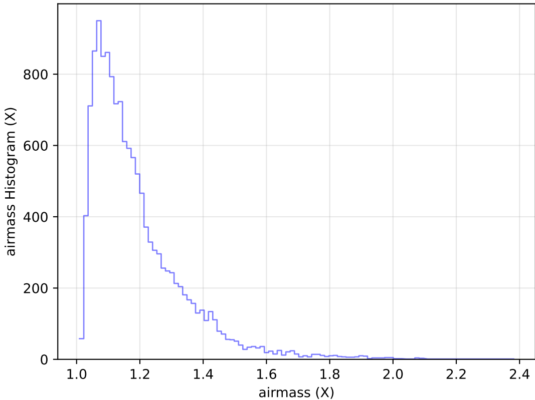
baseline_v2.0_10yrs Yr 1 u band: airmass Histogram
