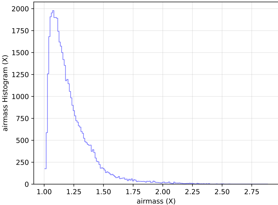
baseline_v2.0_10yrs Yr 1 r band: airmass Histogram
