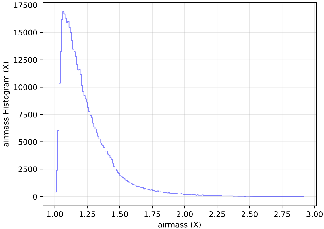
baseline_v2.0_10yrs WFD i band: airmass Histogram
