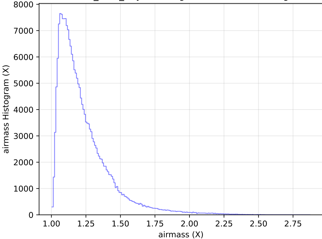
baseline_v2.0_10yrs WFD g band: airmass Histogram
