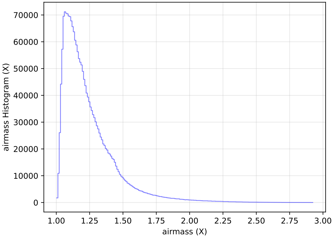
baseline_v2.0_10yrs WFD all bands: airmass Histogram
