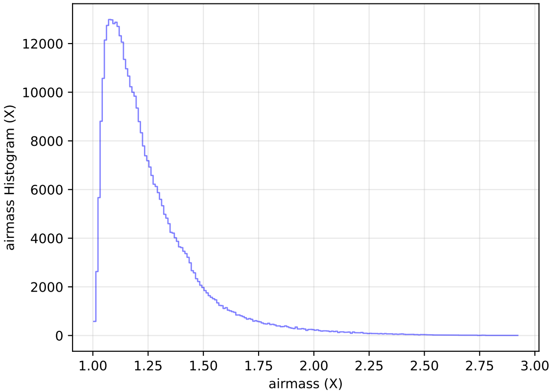
baseline_v2.0_10yrs All sky z band: airmass Histogram
