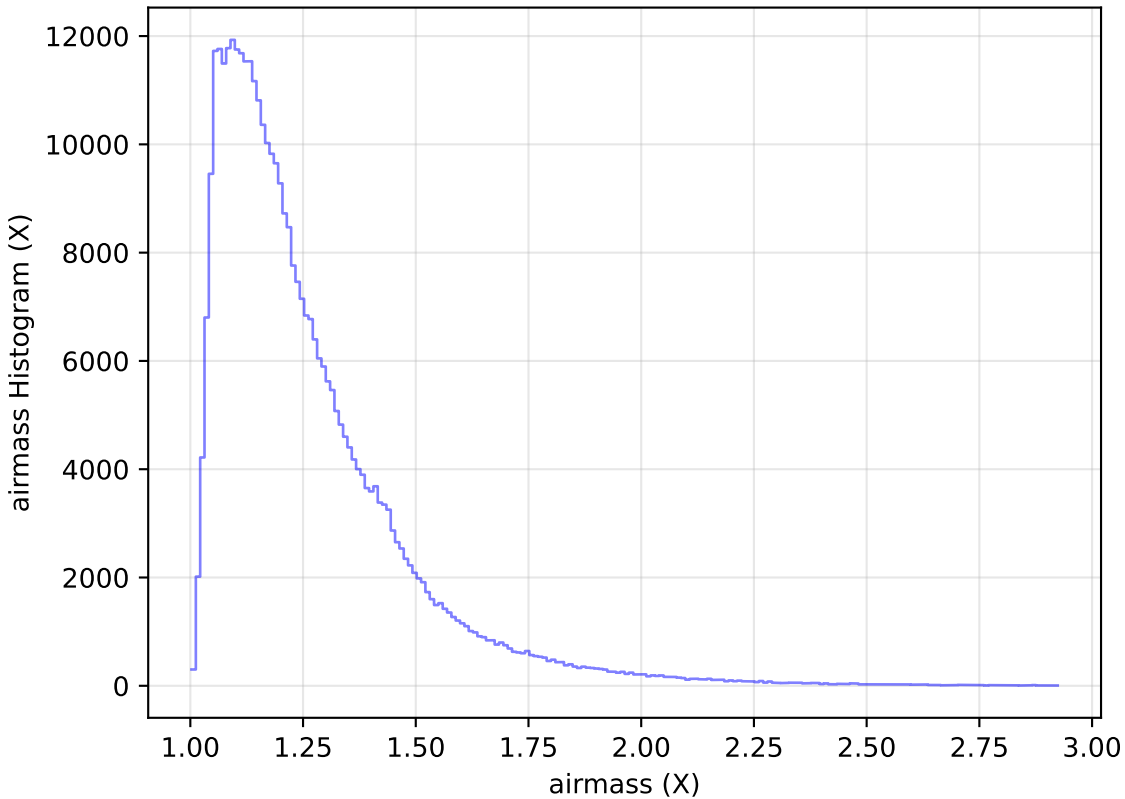
baseline_v2.0_10yrs All sky y band: airmass Histogram
