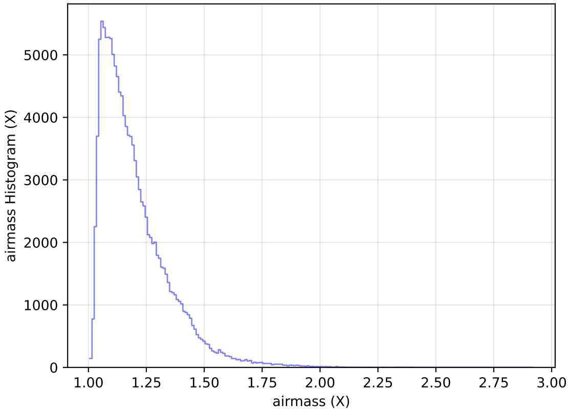
baseline_v2.0_10yrs All sky u band: airmass Histogram
