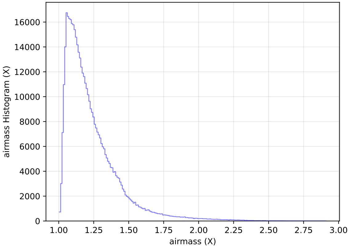
baseline_v2.0_10yrs All sky r band: airmass Histogram
