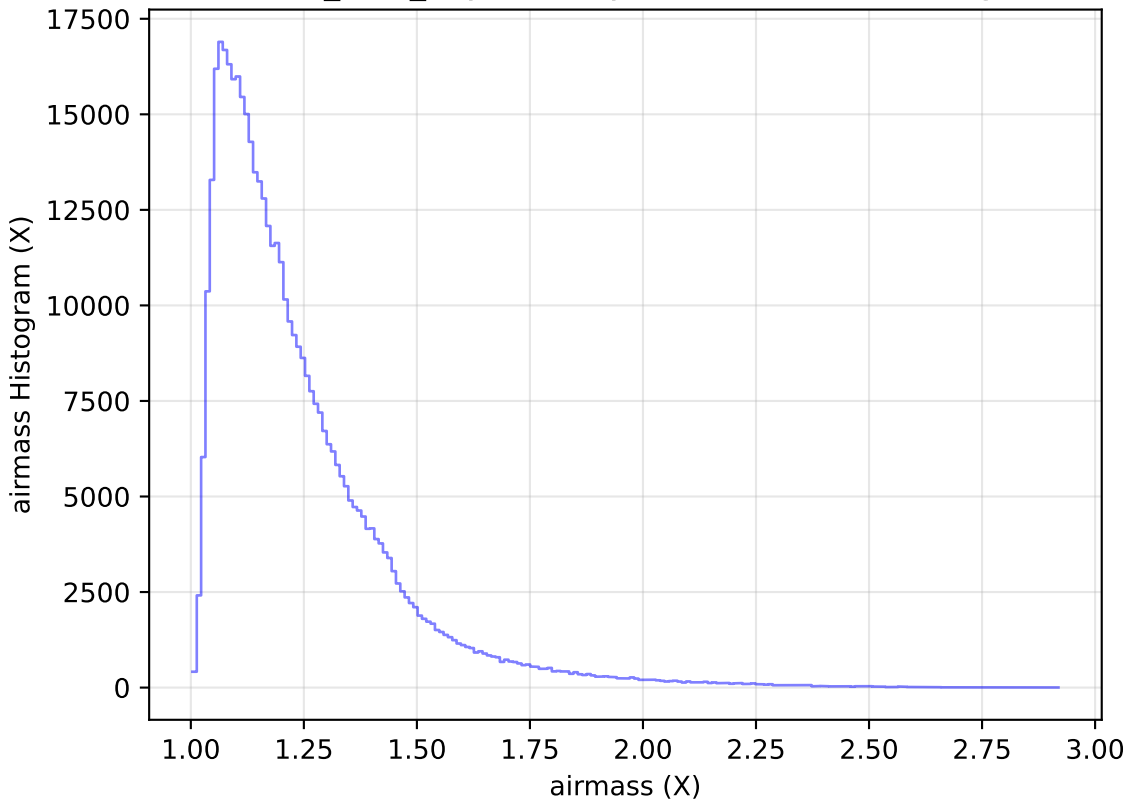
baseline_v2.0_10yrs All sky i band: airmass Histogram
