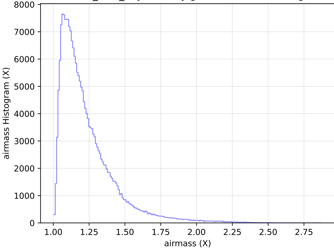
baseline_v2.0_10yrs All sky g band: airmass Histogram
