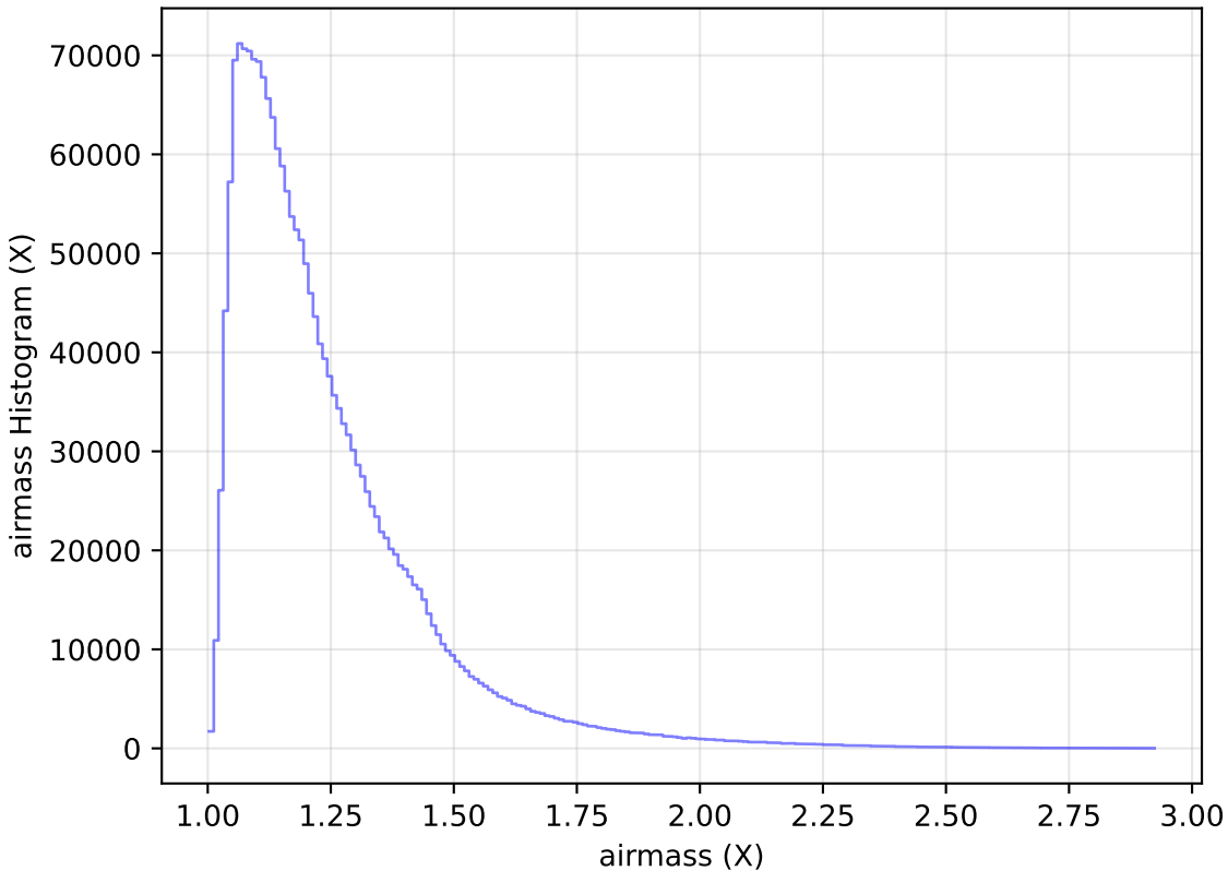
baseline_v2.0_10yrs All sky all bands: airmass Histogram
