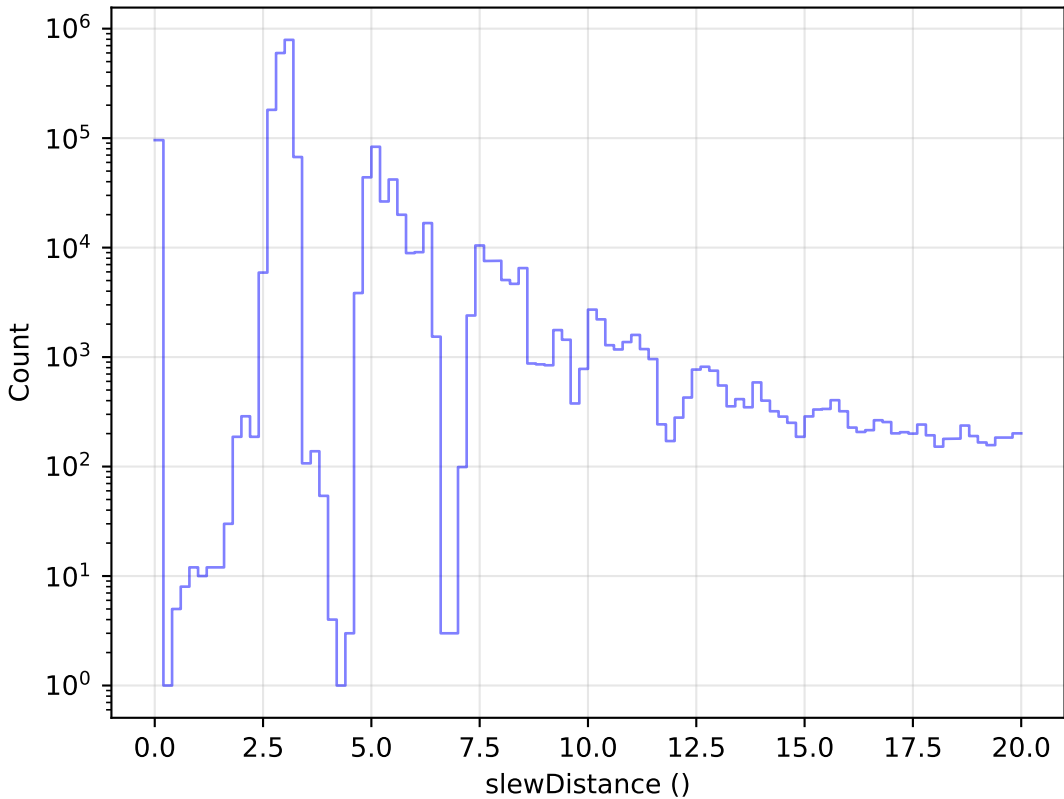
baseline_v2.0_10yrs All visits: Zoom Slew Distance Histogram
