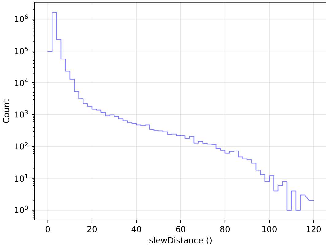
baseline_v2.0_10yrs All visits: Slew Distance Histogram
