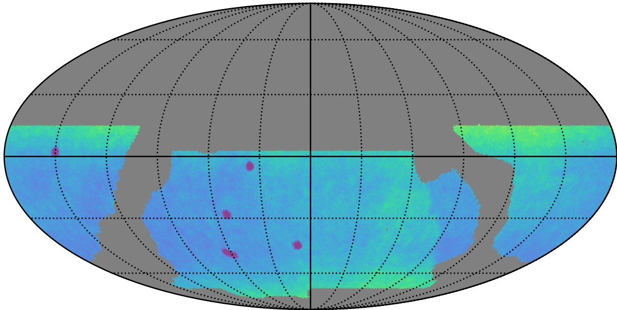
baseline_v2.0_10yrs WFD: Proper Motion Uncert @ 24.0
