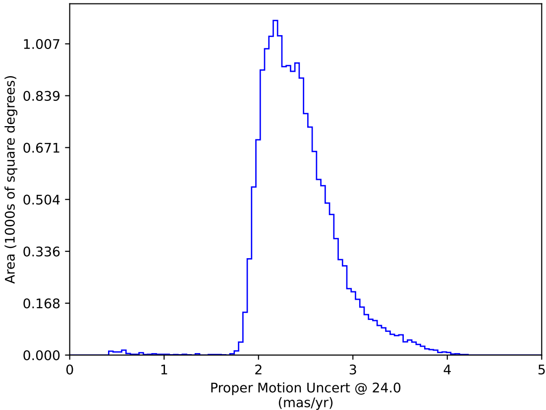
baseline_v2.0_10yrs WFD: Proper Motion Uncert @ 24.0
