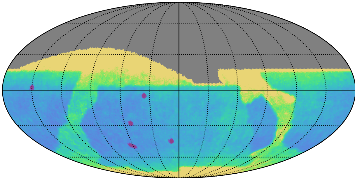
baseline_v2.0_10yrs All sky: Proper Motion Uncert @ 24.0
