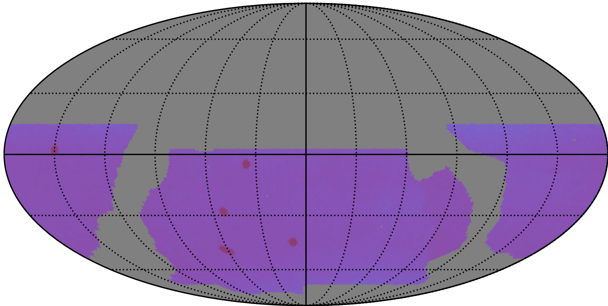
baseline_v2.0_10yrs WFD: Proper Motion Uncert @ 20.5
