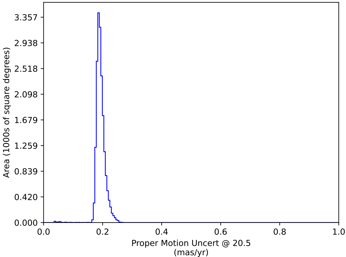
baseline_v2.0_10yrs WFD: Proper Motion Uncert @ 20.5
