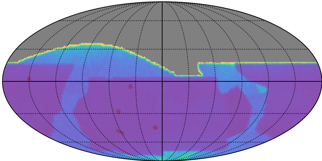
baseline_v2.0_10yrs All sky: Proper Motion Uncert @ 20.5
