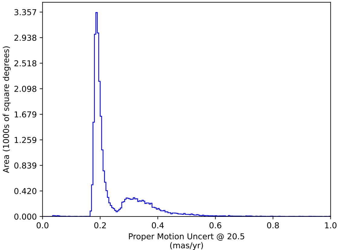
baseline_v2.0_10yrs All sky: Proper Motion Uncert @ 20.5
