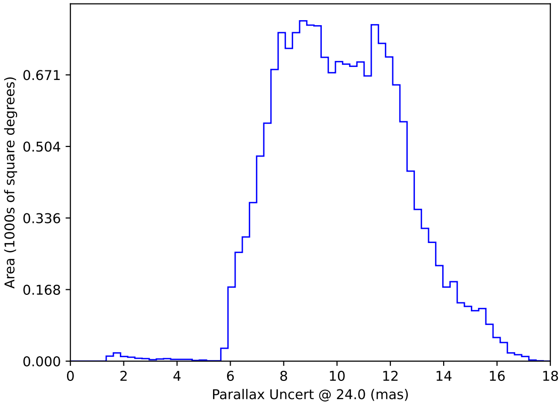
baseline_v2.0_10yrs WFD: Parallax Uncert @ 24.0
