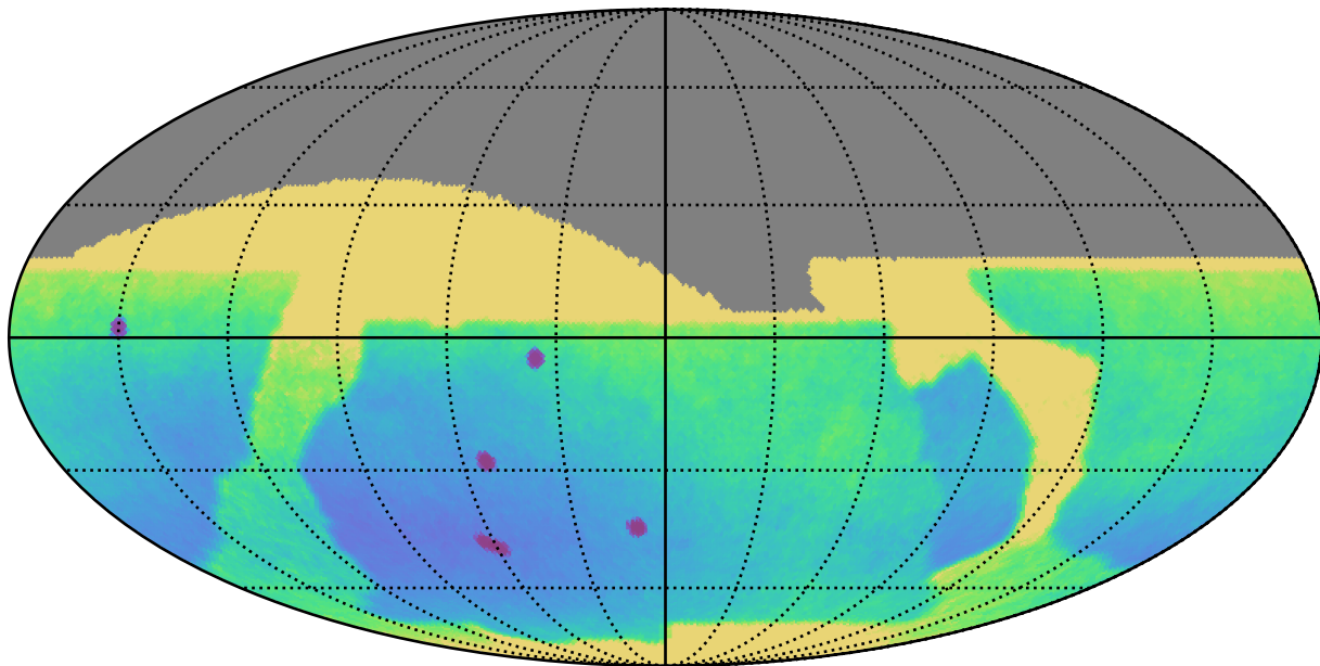
baseline_v2.0_10yrs All sky: Parallax Uncert @ 24.0
