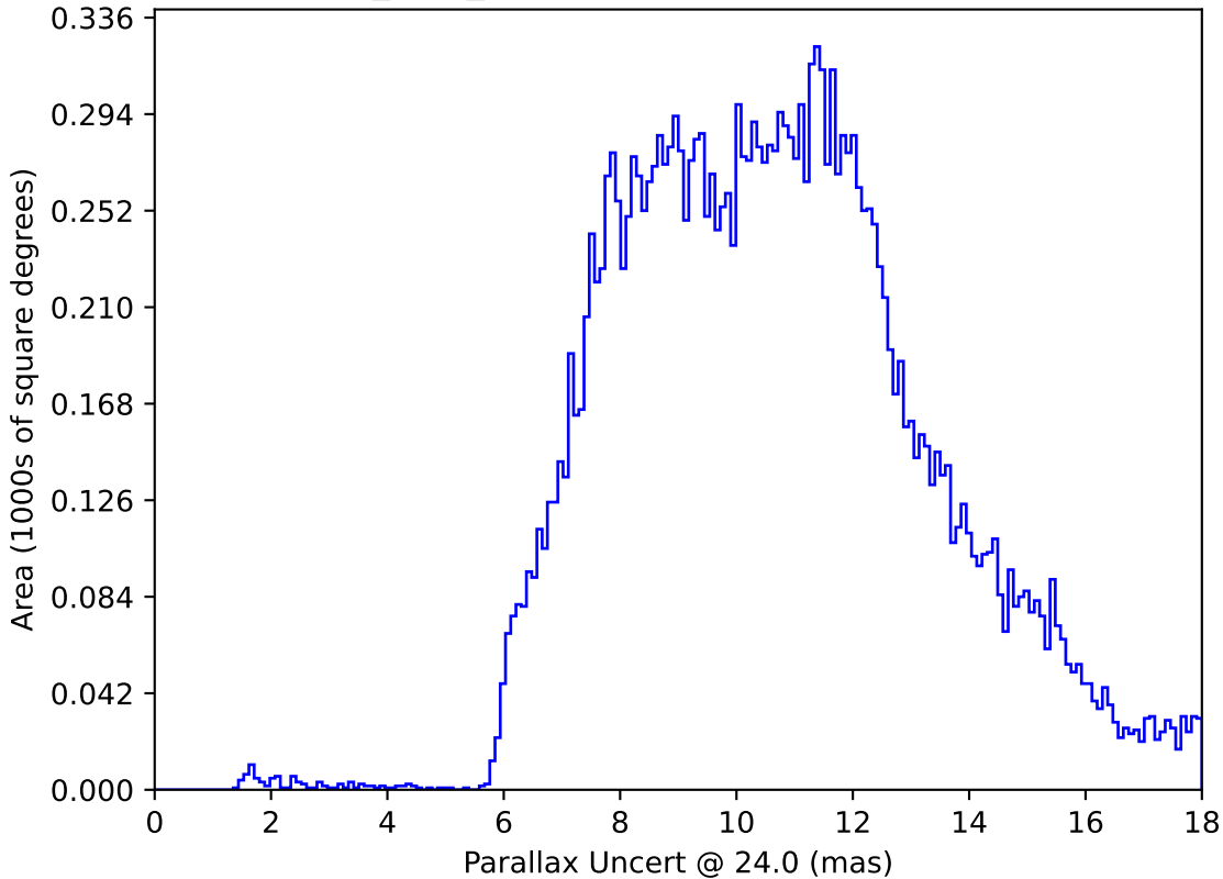
baseline_v2.0_10yrs All sky: Parallax Uncert @ 24.0
