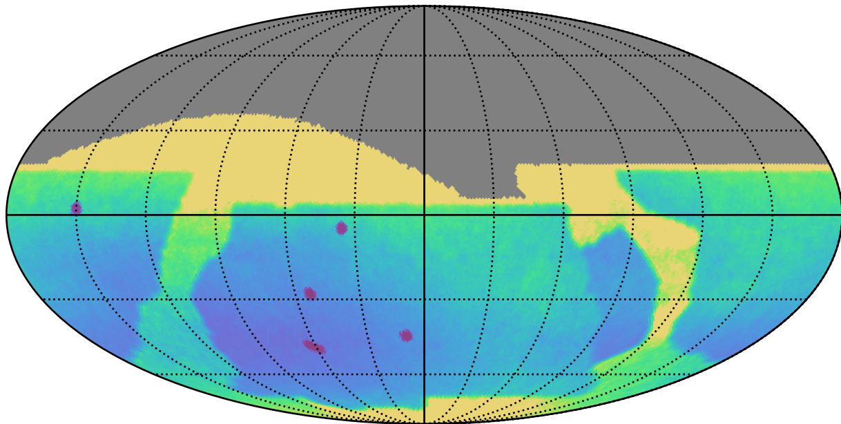
baseline_v2.0_10yrs All sky: Parallax Uncert @ 22.4
