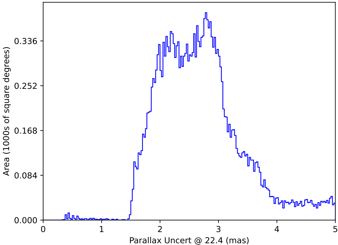
baseline_v2.0_10yrs All sky: Parallax Uncert @ 22.4
