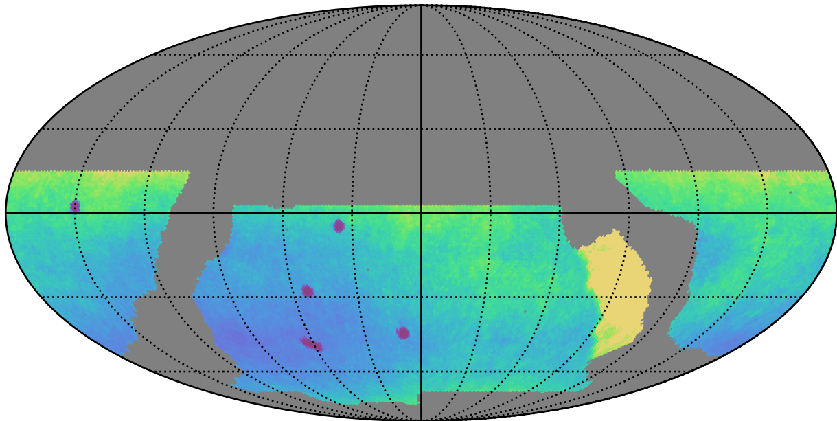
baseline_v2.0_10yrs WFD y band only: Parallax Uncert @ 21.3
