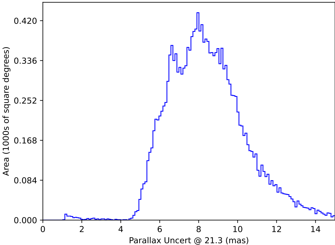
baseline_v2.0_10yrs WFD y band only: Parallax Uncert @ 21.3
