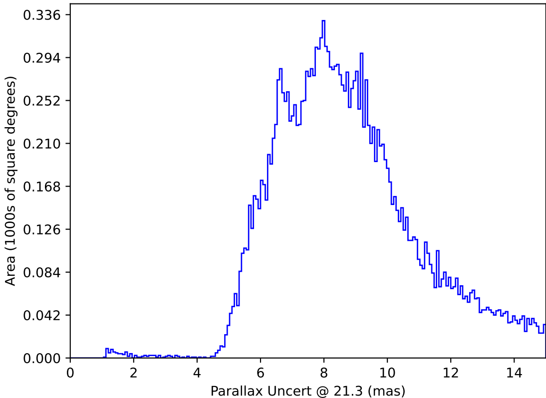
baseline_v2.0_10yrs All sky y band only: Parallax Uncert @ 21.3
