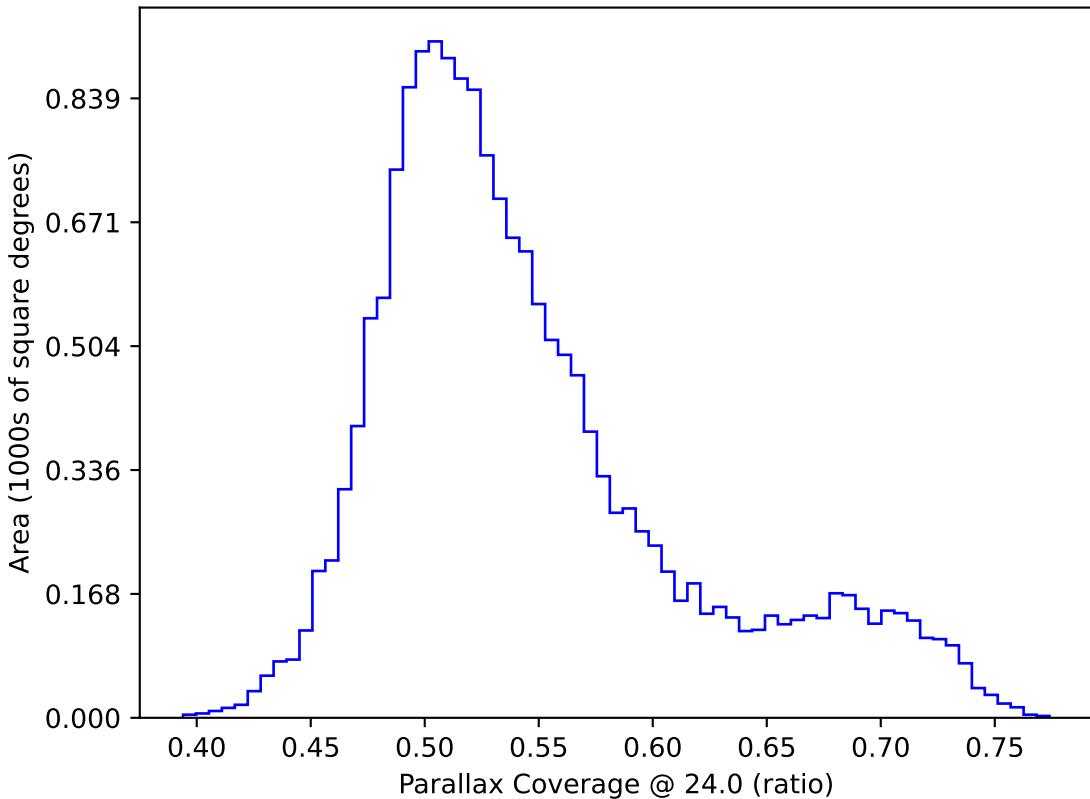
baseline_v2.0_10yrs WFD: Parallax Coverage @ 24.0
