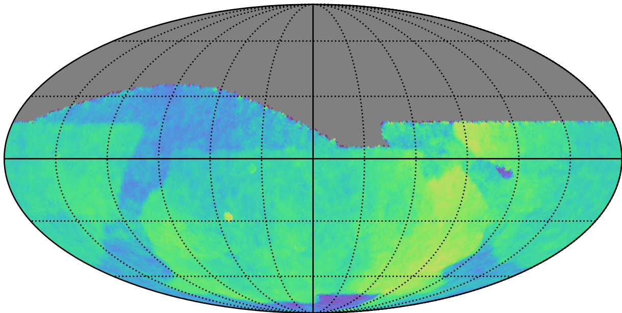
baseline_v2.0_10yrs All sky: Parallax Coverage @ 24.0
