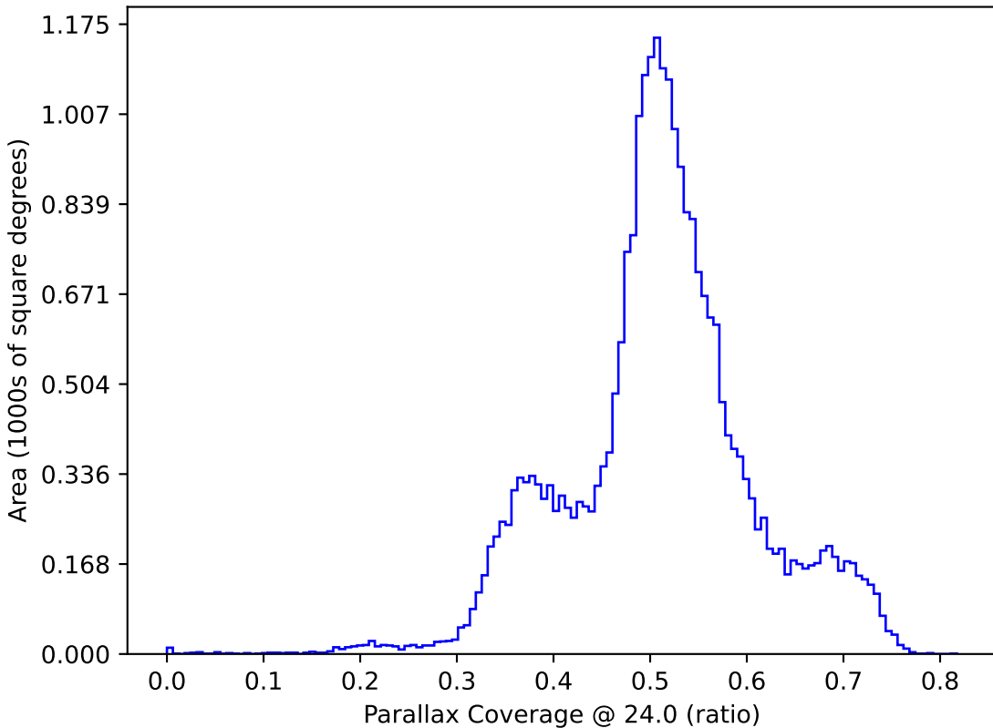
baseline_v2.0_10yrs All sky: Parallax Coverage @ 24.0
